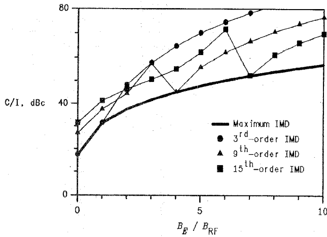
Fig. 3. IMD levels for finite envelope bandwidth (theory).
