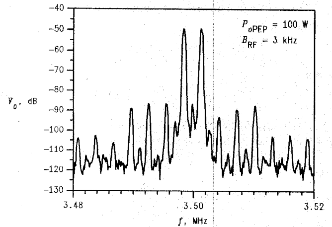
Fig. 5. Measured IMD spectrum for voice-bandwidth test signal.
