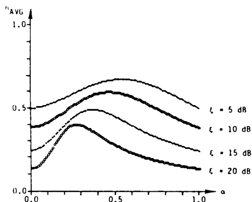
Figure 8. Average efficiency with Laplacian signals or envelopes.
