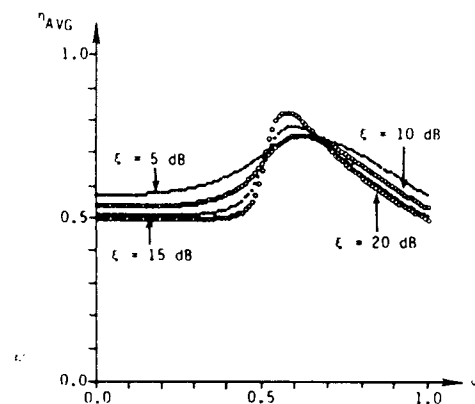
Figure 10. Average efficiency with Laplacian modulation.
