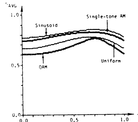
Figure 5. Average efficiency with selected signals.
