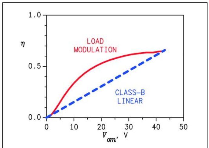
Figure 71 · Instantaneous efficiency of load modulation compared to class-B linear amplification.
