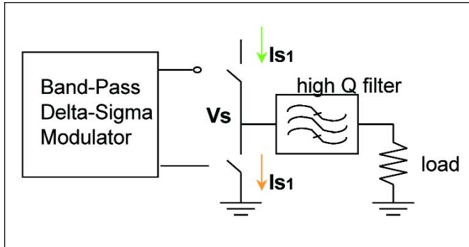
Figure 63 · Delta-sigma modulator.
