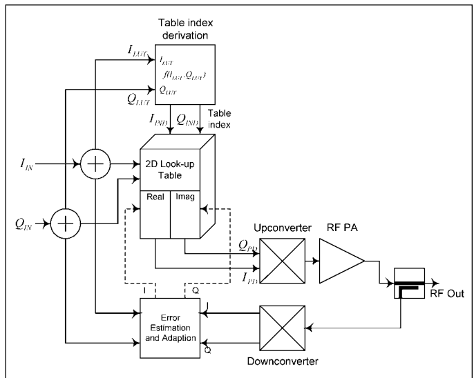
Figure 53 · Mapping predistorter.
