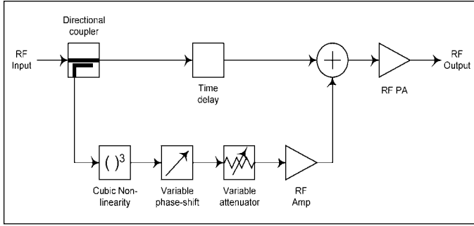
Figure 51 · An RF predistorter.
