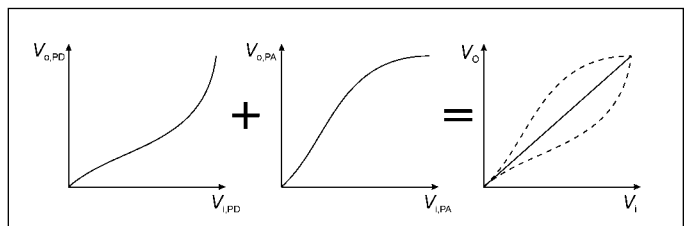
Figure 50 · Amplitude correction by predistortion.
