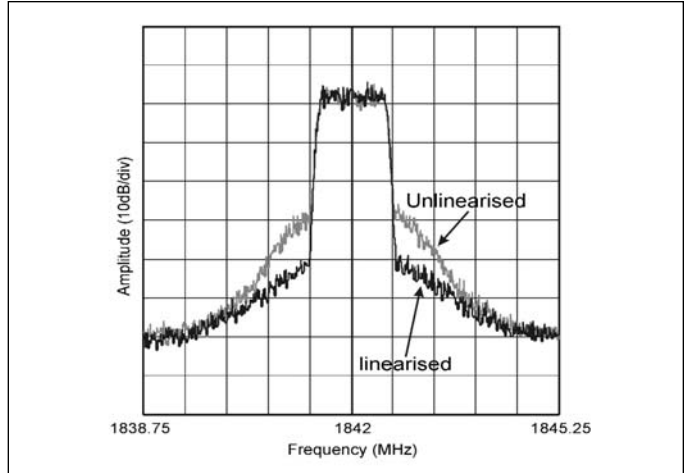
Figure 52 · Linearization by diode-based RF predistorter (courtesy WSI).
