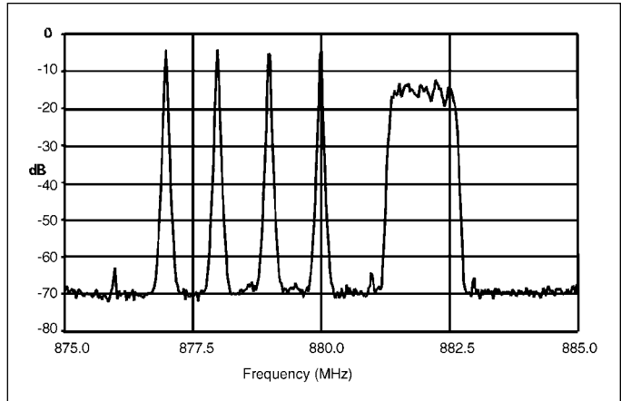
Figure 48 · Feedforward performance with mixed-mode modulation (TDMA and CDMA signals).
