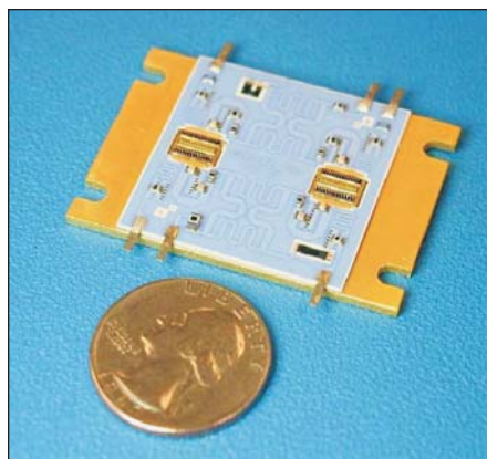
Figure 18 · Thick-film hybrid S-band PA module. (Courtesy UltraRF)
