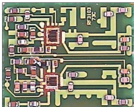
Figure 17 · Internal view of a dual-band (GSM/DCS) PA module for cellular telephone handsets. (Courtesy RF Micro Devices)
