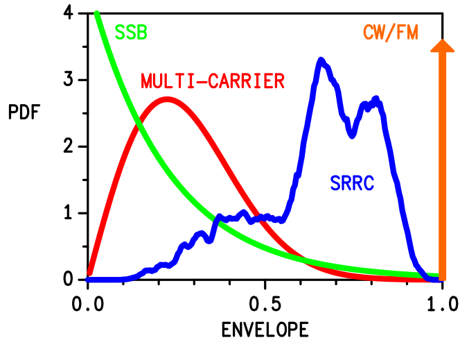
Figure 2. Signal probability densities.
